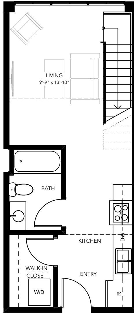
FIRST FLOOR
